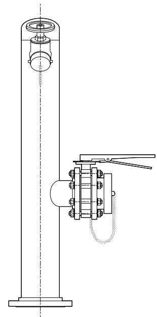
Figure 2 Typical Wet Barrel Hydrant Header
